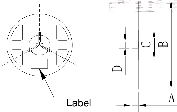
Fig.2-2 Reel Dimension
