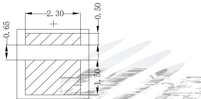
Fig.1-3 Bottom View
