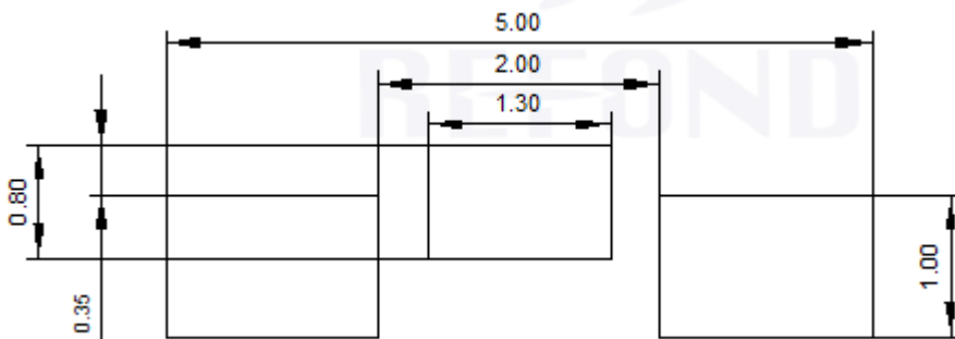
Fig.1-5 Soldering patterns
