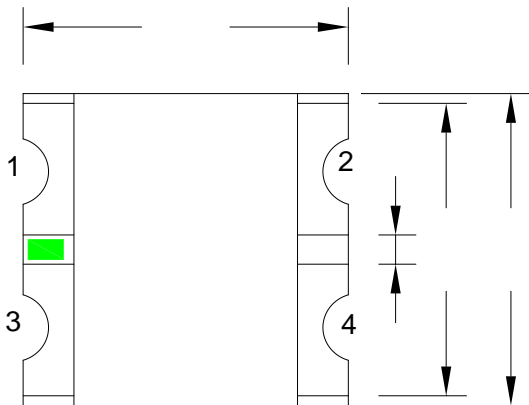
Fig.1-1 Top view
