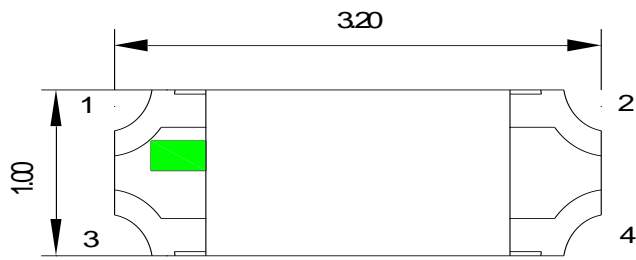
Fig.1-1 Top view
