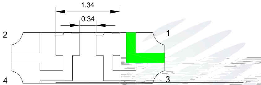
Fig.1-3 Bottom view
