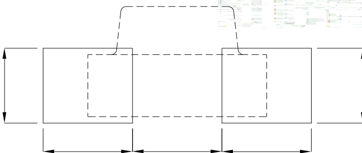
Fig.1-5 Soldering patterns 推荐焊盘
